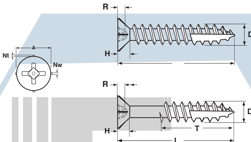
SQUARE-PHILLIPS COMBO FLAT HEAD DEEP THREAD WOOD SCREW—TYPE-17 WITH NIBS
