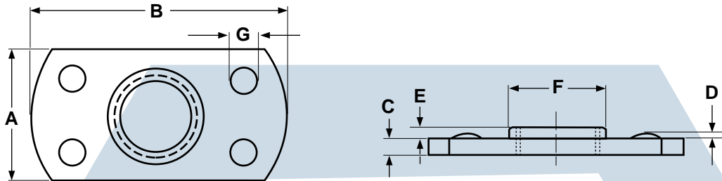
TAB WELD NUTS - CENTER HOLE DESIGN WITH MULTIPLE PROJECTIONS
