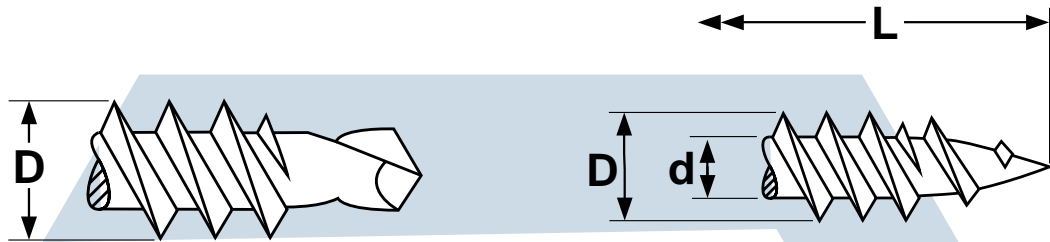
Fine Thread Drill Point Drywall Screw
